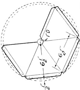
Pattern for Screen
